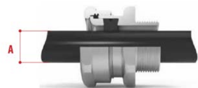
Cable gland with gasket with unarmored cable
